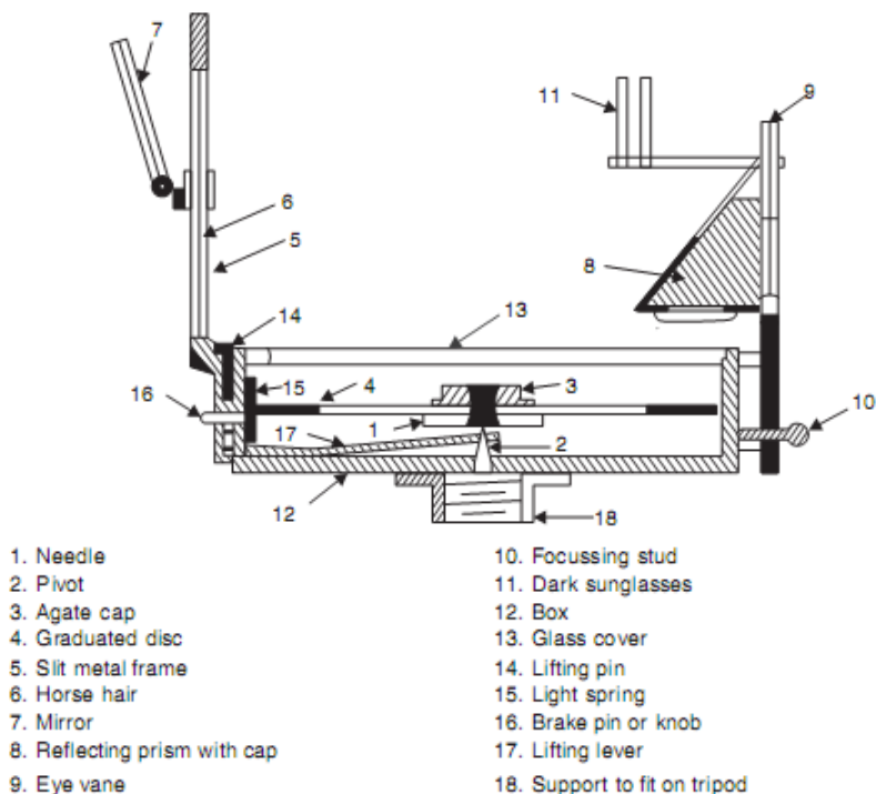
Fig. 13.1. Prismatic compass
